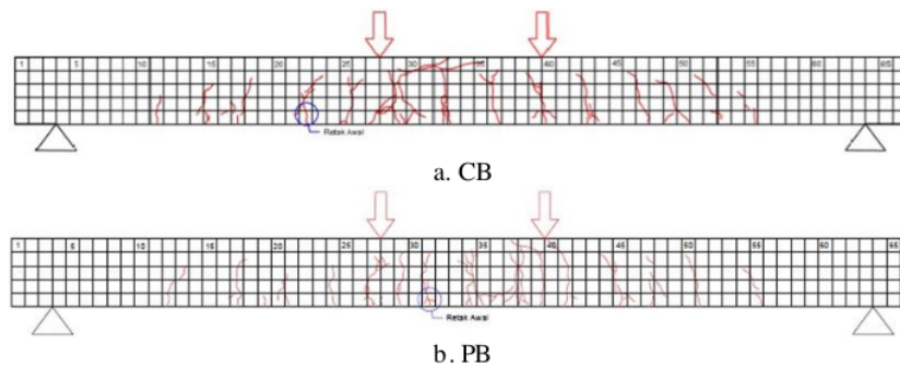
Figure 9 Crack pattern
