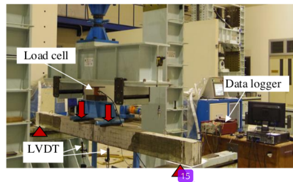
Figure 4 Loading test
